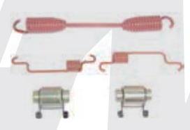
KRB-K5481 Universal Kit for Eaton ES Extended Service Brake, Includes: 2 retainer spring, 2 roller, 2 roller retainer, 2 brake return spring
