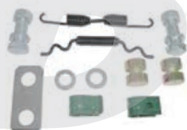
KRB-K3869 Universal Kit for Rockwell "Q" Series 15x4 Front Brake. Includes: 2 shoe clip, 2 roller, 2 anchor pin, 1 retainer spring, 1 return spring, 2 anchor pin washer, 1 anchor pin plate, 1 anchor pin lock nut
